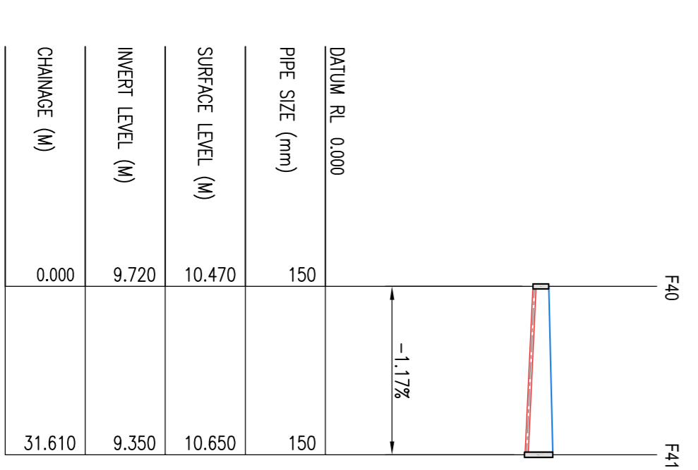
LONGITUDINAL SECTION FROM MANHOLE F40 TO F41 SCALES - 1:1000 H 1:250 V
