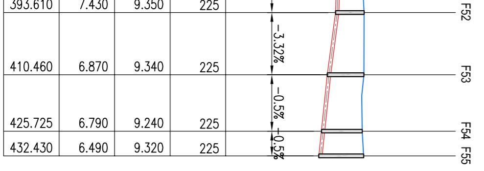
LONGITUDINAL SECTION FROM MANHOLE F49 TO F51 SCALES - 1:1000 H 1:250 V
