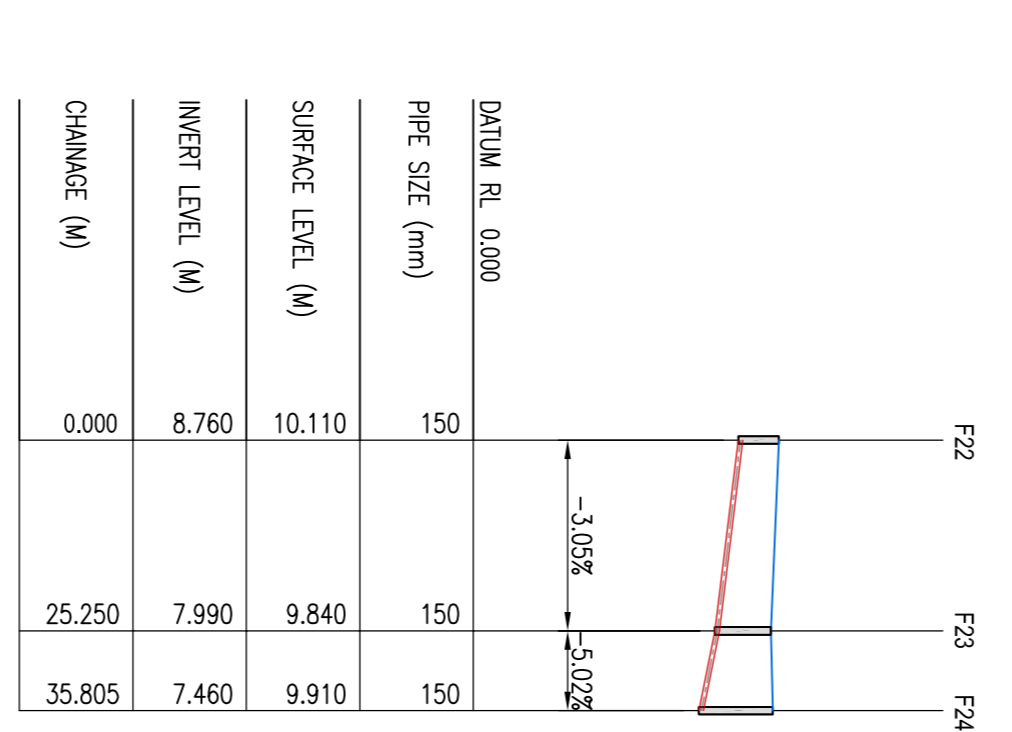
LONGITUDINAL SECTION FROM MANHOLE F22 TO F24 SCALES - 1:1000 H 1:250 V
