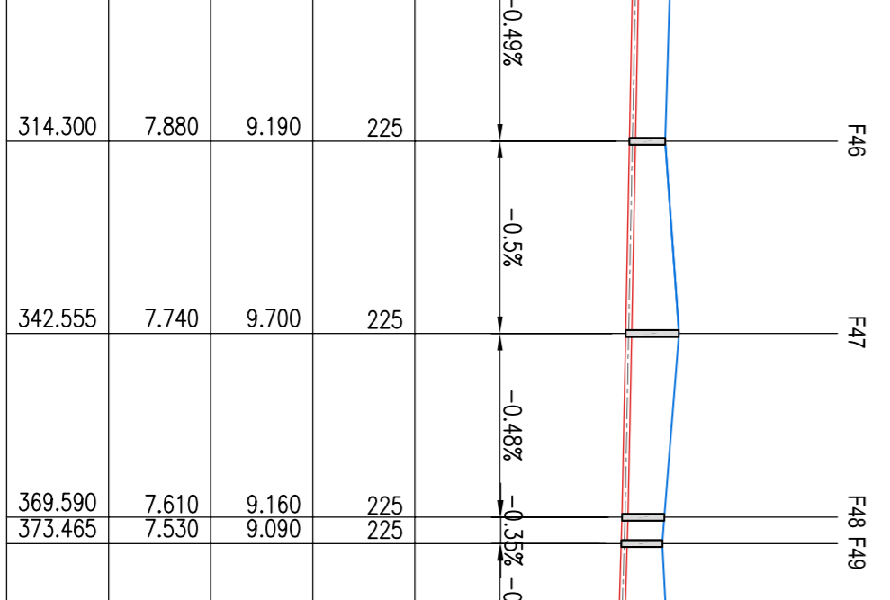
LONGITUDINAL SECTION FROM MANHOLE F46 TO F49 SCALES - 1:1000 H 1:250 V
