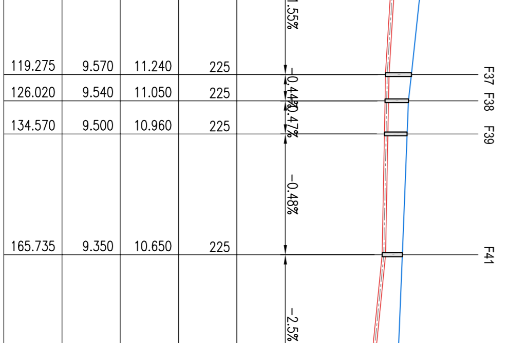
LONGITUDINAL SECTION FROM MANHOLE F37 TO F41 SCALES - 1:1000 H 1:250 V
