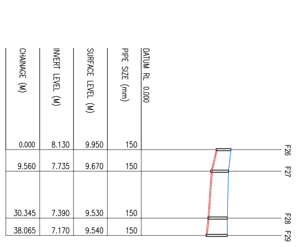
LONGITUDINAL SECTION FROM MANHOLE F26 TO F29 SCALES - 1:1000 H 1:250 V
