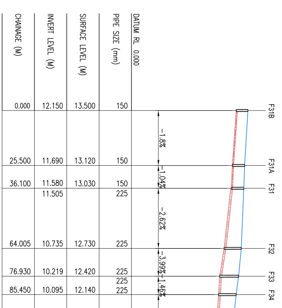
LONGITUDINAL SECTION FROM MANHOLE F31 TO F35 SCALES - 1:1000 H 1:250 V
