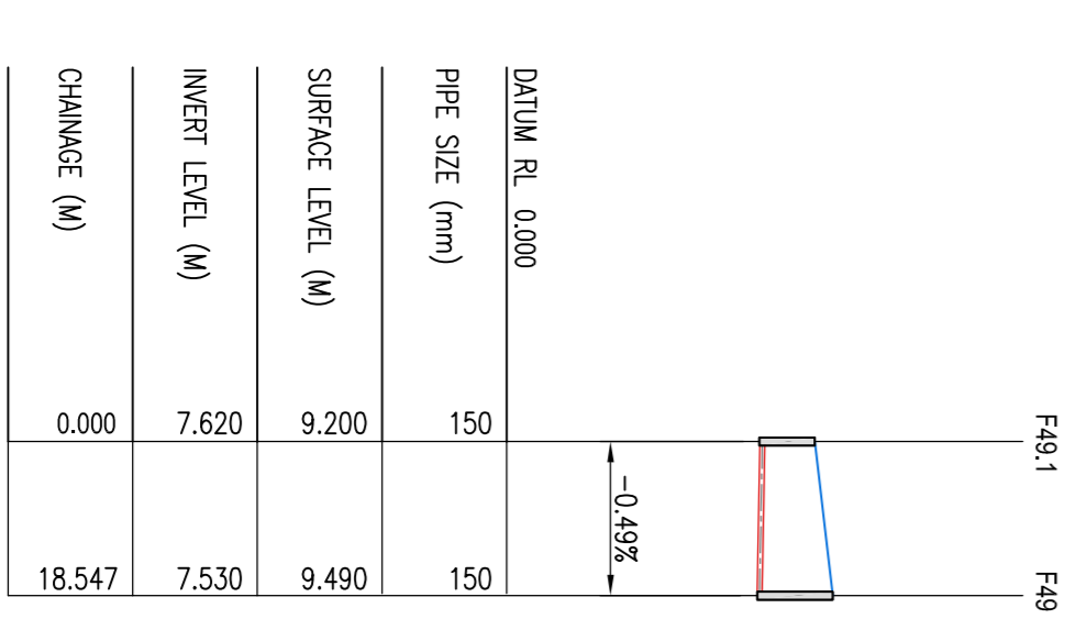
LONGITUDINAL SECTION FROM MANHOLE F49 TO F49.1 SCALES - 1:1000 H 1:250 V
