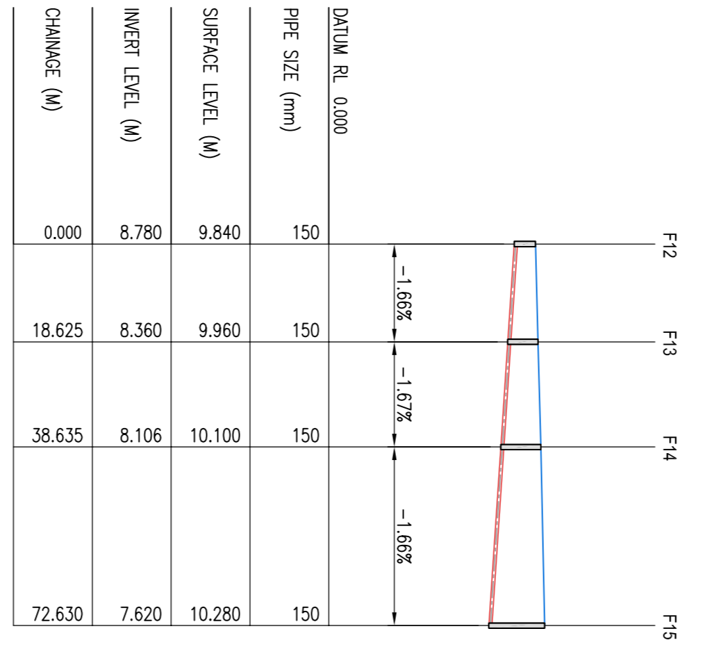
LONGITUDINAL SECTION FROM MANHOLE F12 TO F15 SCALES - 1:1000 H 1:250 V
